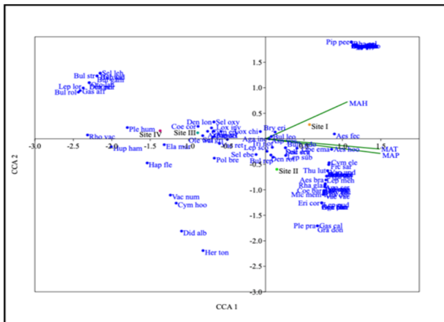
Figure 7. Canonical correspondence analysis (CCA) plot showing the influence of environmental variables
